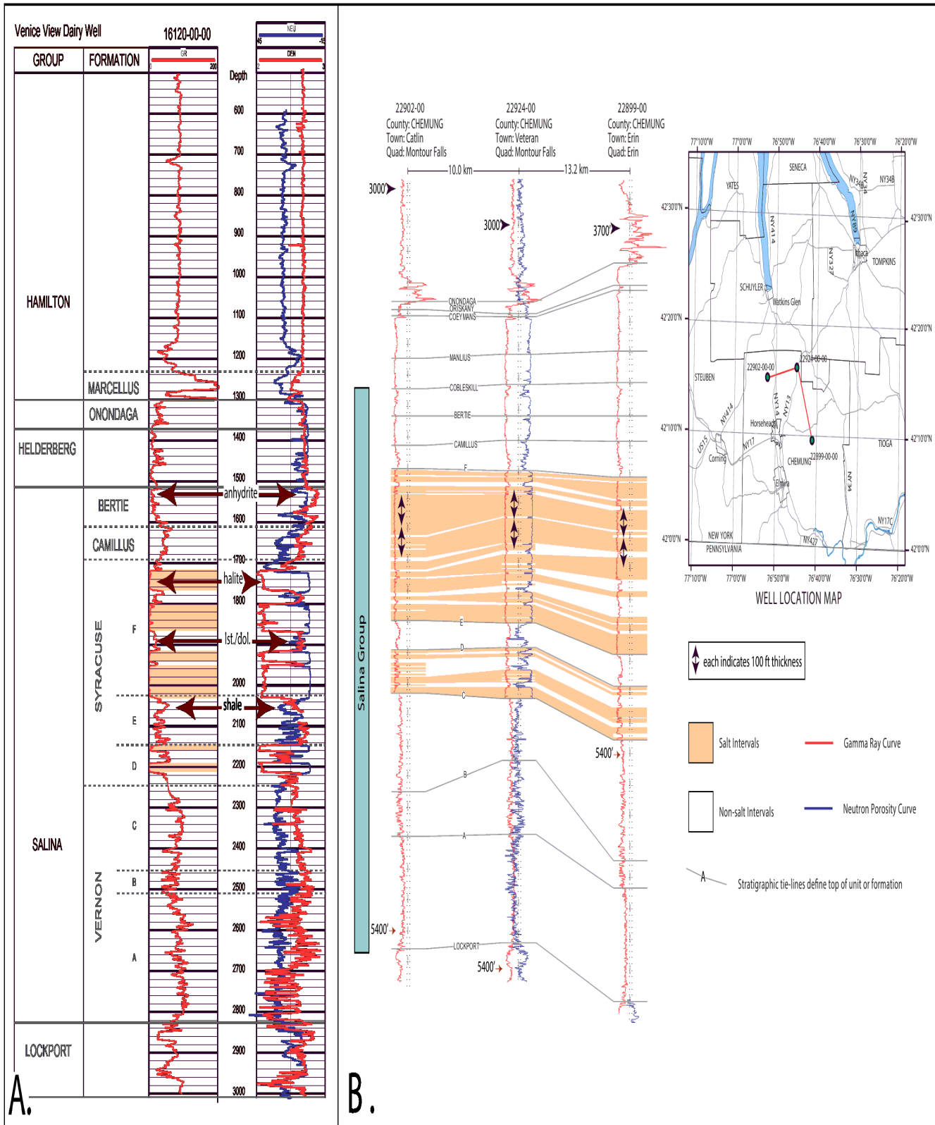
Figure 7 Wireline character of the Syracuse Formation. A) Wireline interpretation of salt interval in Venice View Dairy well, with intervals selected to demonstrate wireline determinants of mineralogy (Base log image extracted from Smith et al., 2005). B) Salt correlation panel based on wireline log measures in three wells located south of Cayuga Lake (base images extracted from Smith et al., 2005).
