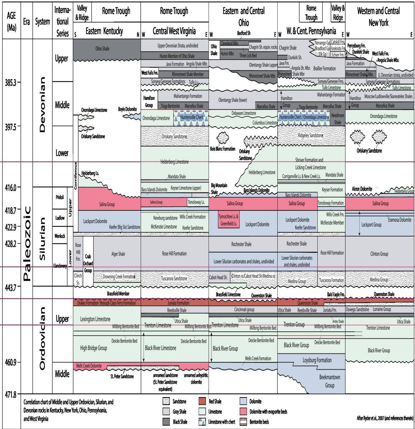
Figure 3. Stratigraphic correlation panel showing how the rock unit names vary across the region, but the evaporitic Salina Group is regionally extensive (extracted from Ryder et al., 2007)
